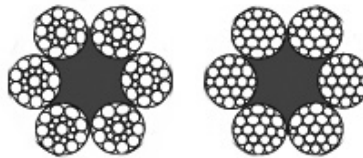
6 x 19 Classification + Fibre core (CFN)
