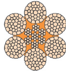
Powerform 6P
